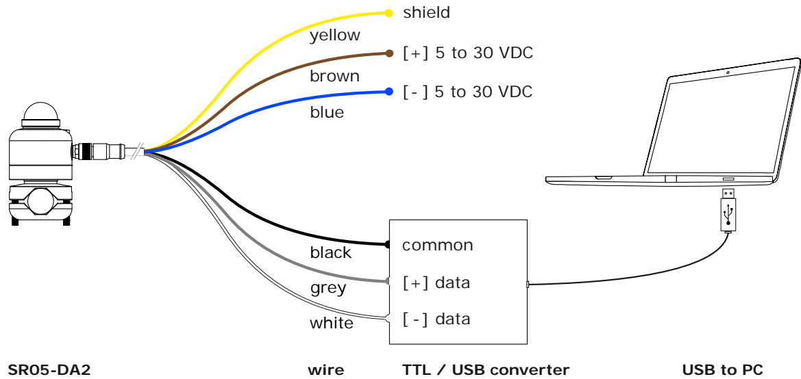
Figure 5.12.2.1 Connecting SR05-DA2 to a TTL to USB converter and a PC
