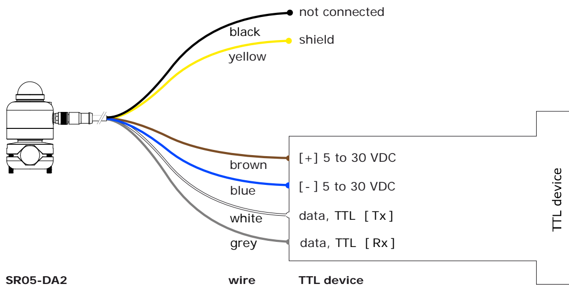
Figure 5.11.2 Connection of SR05-DA2 to a TTL device, in case SR05-DA2 is powered by the read-out device itself.
