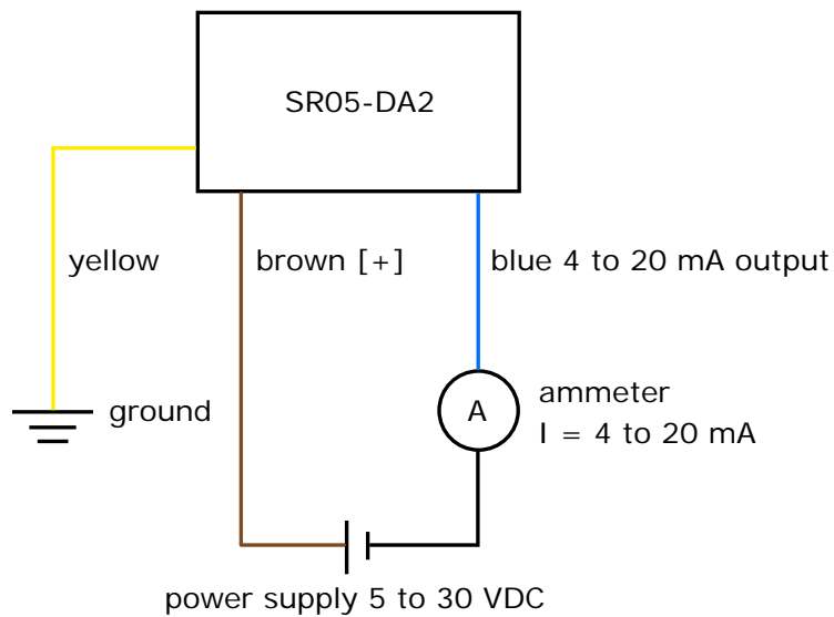
Figure 5.8.1 Electrical diagram of the connection of SR05-DA2 to a typical ammeter or datalogger with capacity to measure current signals. SR05-DA2 operates on a supply voltage of 5 to 30 VDC.
