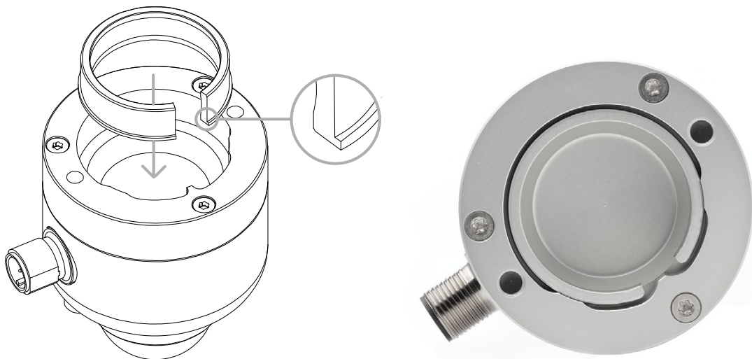
Figure 9.4.1 Line drawing indicating placement of the aluminium shim and photo showing the shim properly positioned in the centre of SR05's bottom plate. Note the position of the protruding ledge when placing the shim.
