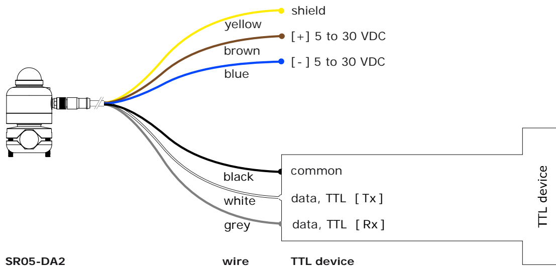
Figure 5.11.1 Connection of SR05-DA2 to a TTL device, in case SR05-DA2 is powered by an external power supply of 5 to 30 VDC.
