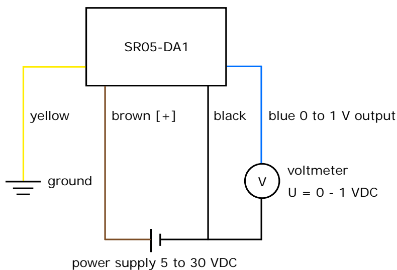
Figure 5.7.1 Electrical diagram of the connection of SR05-DA1 to a typical voltmeter or datalogger with the capacity to measure voltage signals. SR05-DA1 operates on a supply voltage of 5 to 30 VDC.
