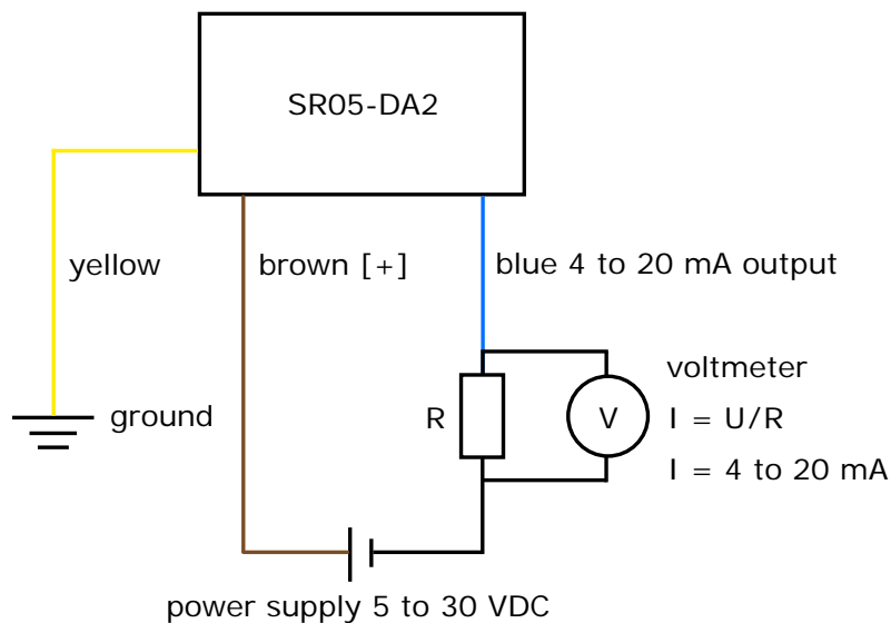
Figure 5.8.2 Electrical diagram of the connection of SR05-DA2 to a typical voltmeter or datalogger with the capacity to measure voltage signals. Usually a 100 \Omega shunt resistor ( R ) is used to convert the current to a voltage. SR05-DA2 operates on a supply voltage of 5 to 30 VDC.
