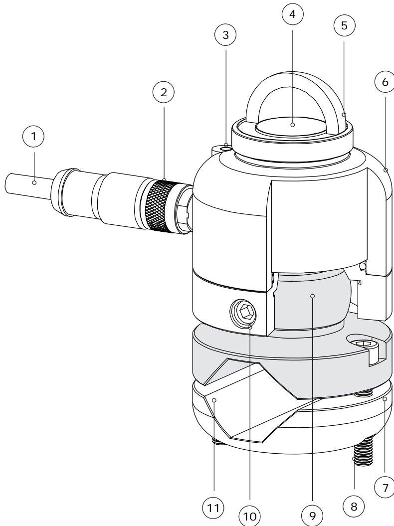
Figure 2.1 Overview of SR05: Shaded area in exploded view shows ball levelling mount
