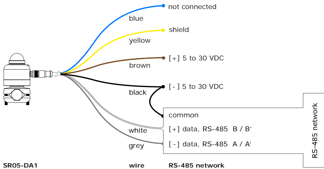
Figure 5.10.2 Connection of SR05-DA1 to an RS-485 network. SR05-DA1 is powered by an external power supply of 5 to 30 VDC.
