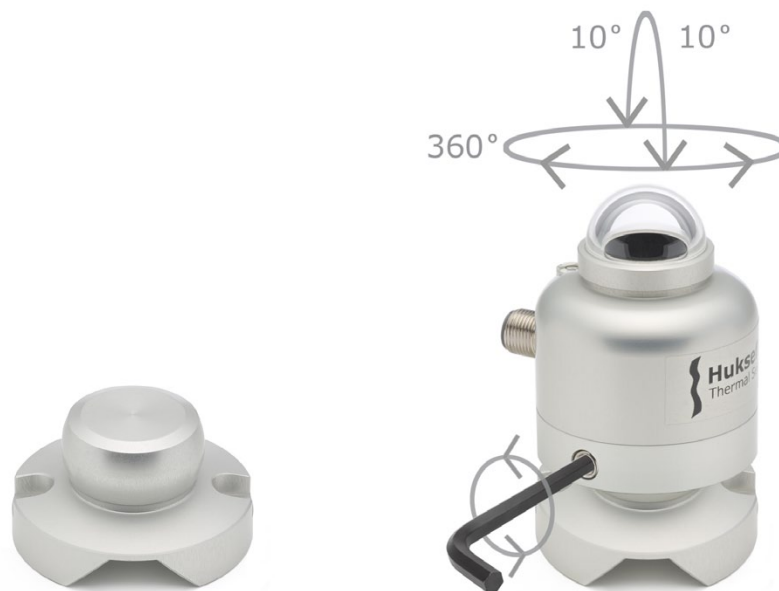
Figure 5.4.1 On the left SR05's ball levelling (mounting screws not displayed) and on the right SR05 placed on the ball levelling mount. Loosen the countersunk set screw on SR05's side to unlock, allowing placement of the ball head and SR05 levelling, and tighten it to lock the ball head mechanism. A 4 mm hex key is the only tool needed to place and remove the ball levelling and to allow and disallow levelling adjustment.
